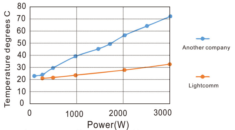
End Cap end Face max Temp vs Power
