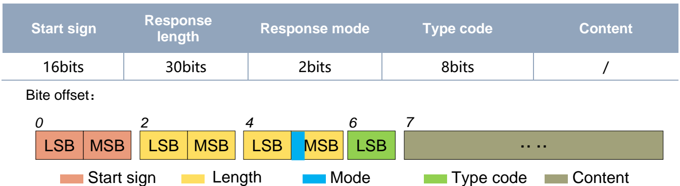
FIG 3 YDLIDAR TG SERIES SYSTEM MESSAGE DATA PROTOCOL
