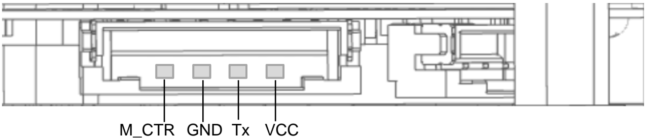
FIG 3 YDLIDAR X2 INTERFACES
